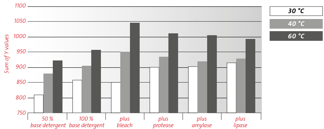
Influence of different washing conditions on the sum of the remission values
